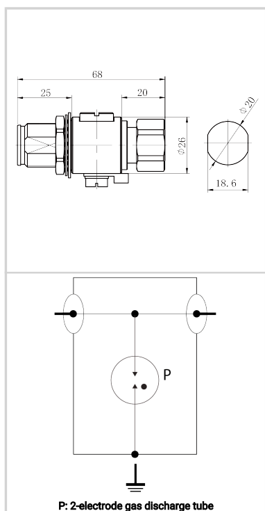
P: 2-electrode gas discharge tube
