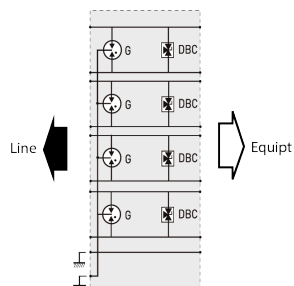
P: 3-electrode GDT DBC: Low capacitance diode
